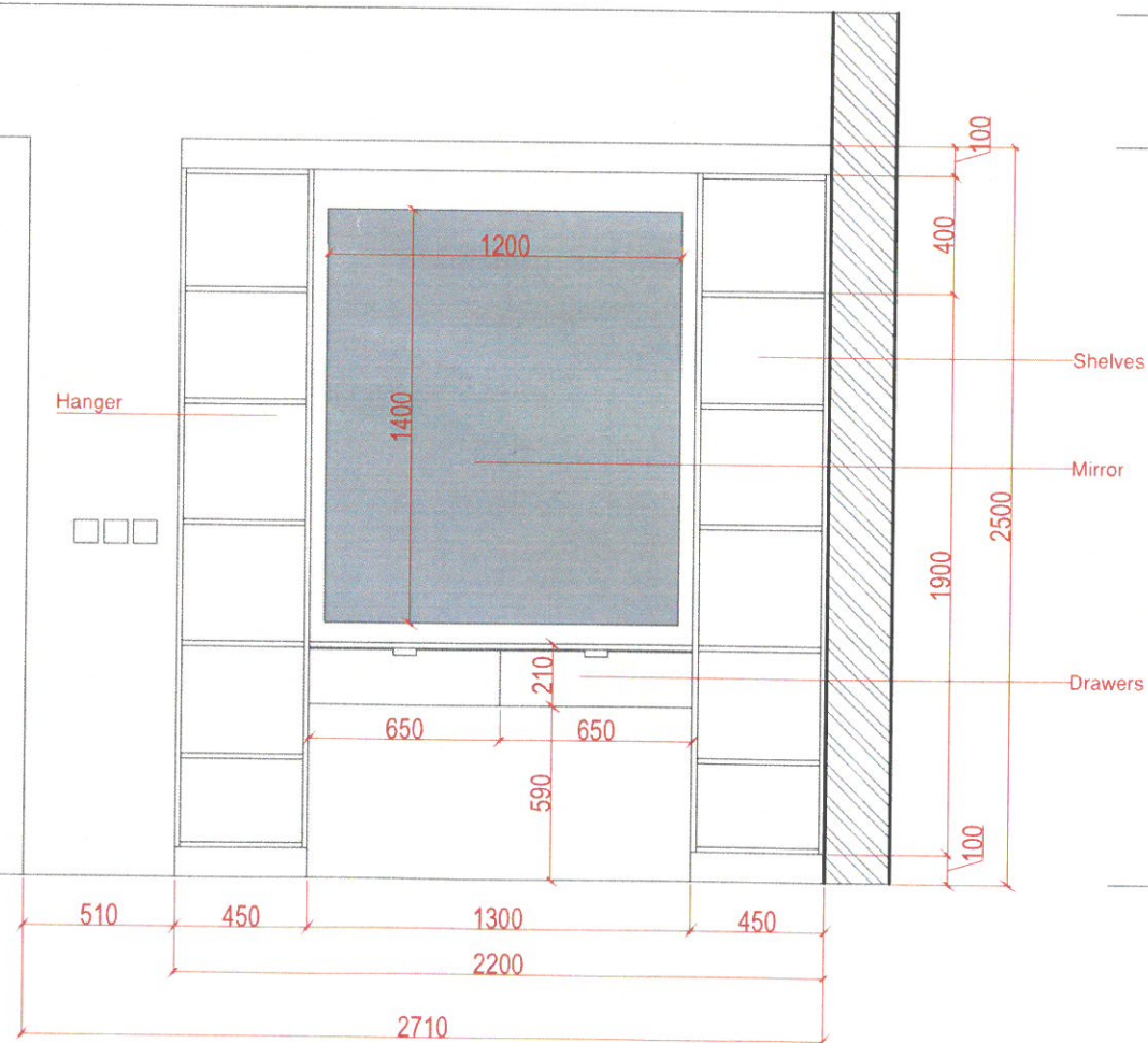
Front Elevations Details
