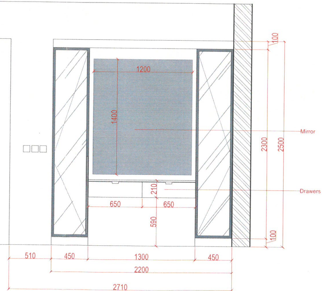
Front Elevation-A Details with Doors
